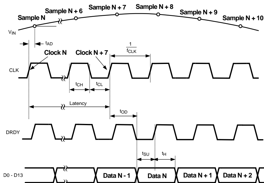
Figure 3. Output Timing
