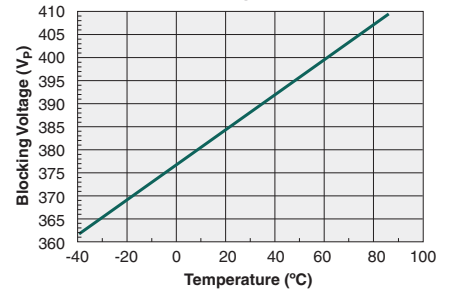
Form-B Typical Blocking Voltage vs. Temperature
