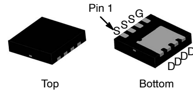
WDFN8 3.3 x 3.3, 0.65P CASE 511DH
