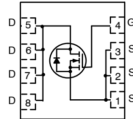
N-CHANNEL MOSFET
