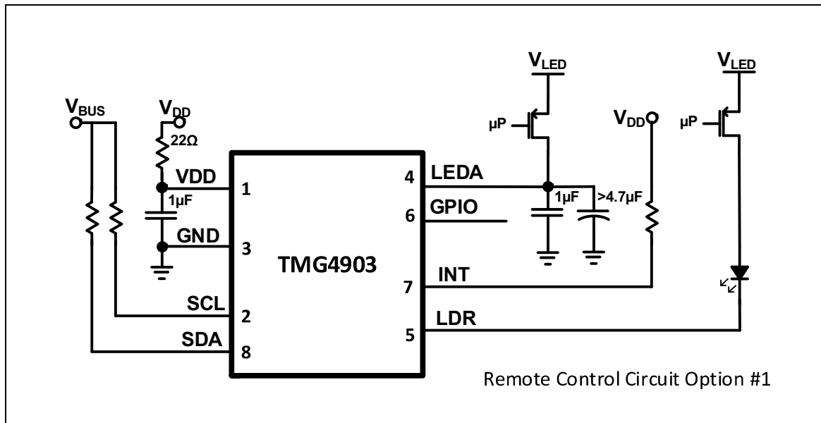
Figure 96: External IR LED Using the LDR Pin
