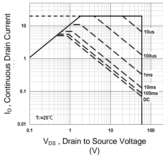
Maximum Safe Operation Area (SOT-223)
