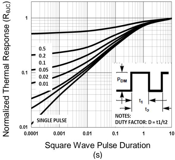
Normalized Transient Impedance (SOT-223)
