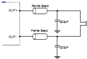
Figure 1: Ferrite Bead Filter to Reduce EMI
