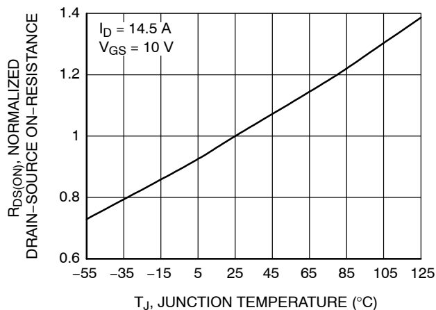
Figure 3. On-Resistance Variation with Junction Temperature
