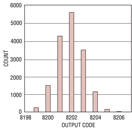
LTC2264-14: Shorted Input Histogram
