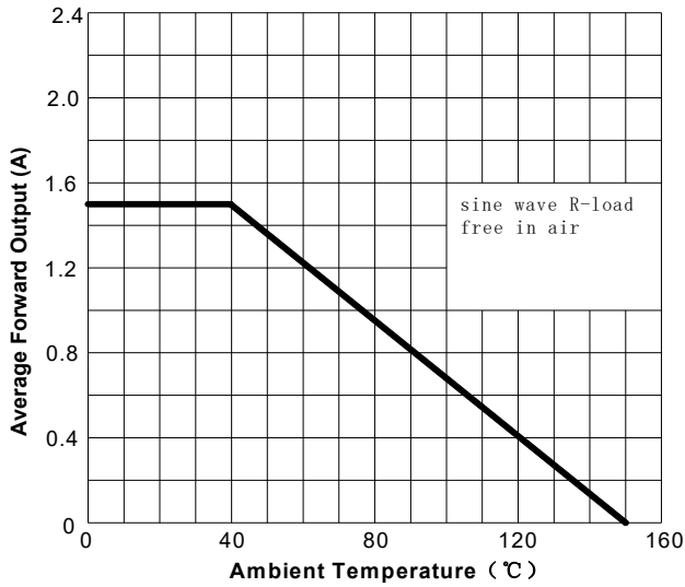
FIG1:Io-Ta Curve
