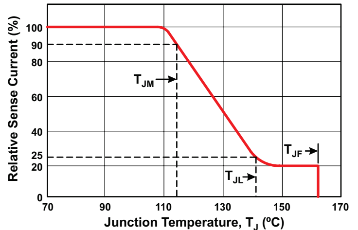
Figure 9: Temperature Monitor Current Reduction
