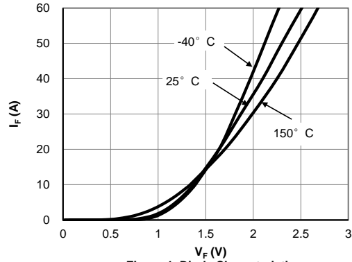
Figure 4: Diode Characteristic
