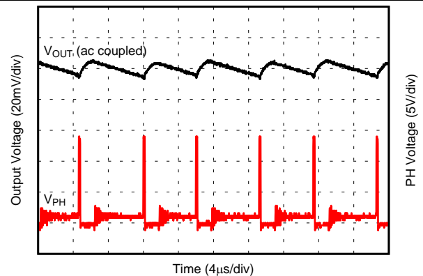
Figure 17. Output Ripple, I_{OUT} = 30 \text{ mA}
