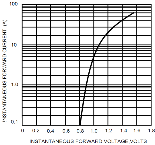
FIG.3-TYPICAL FORWARD CHARACTERISTICS
