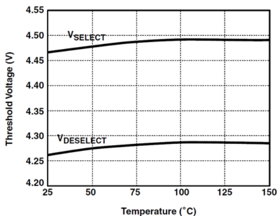
Figure 24. Select/Deselect Threshold Variation with T_{JUNC}
