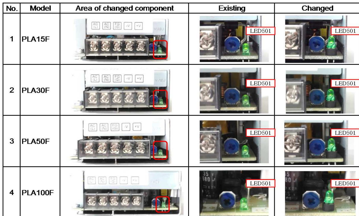
Fig.2.1 Photograph(PLA15F/30F/50F/100F) of "Existing" and "Changed"
