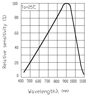
Fig.3 Spectral Sensitivity
