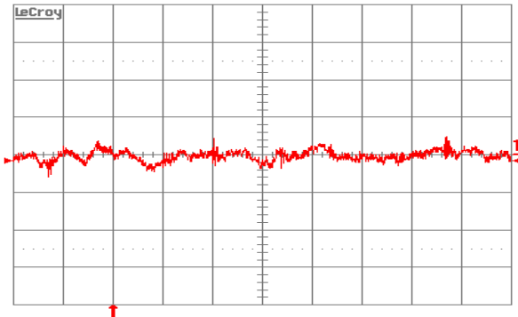
Figure 12. Input reflected-ripple current, i_s (10 mA/div.), measured through 10 \mu H at the source at full rated load current and V_{in} = 48 V. Refer to Figure 11 for test setup. Time scale: 1 \mu s/div.
