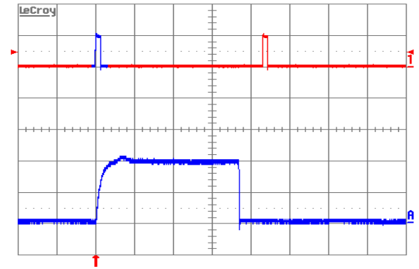
Figure 15. Load current (top trace, 20 A/div., 50 ms/div.) into a 10 m\Omega short circuit during restart, at V_{in} = 48 V. Bottom trace (10 A/div., 2 ms/div.) is an expansion of the on-time portion of the top trace
