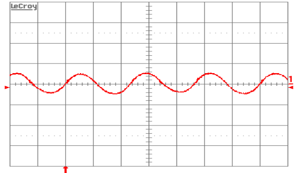
Figure 13. Input reflected ripple-current, i_c (200 mA/div.), measured at input terminals at full rated load current and V_{in} = 48 V. Refer to Figure 11 for test setup. Time scale: 1 \mu s/div.
