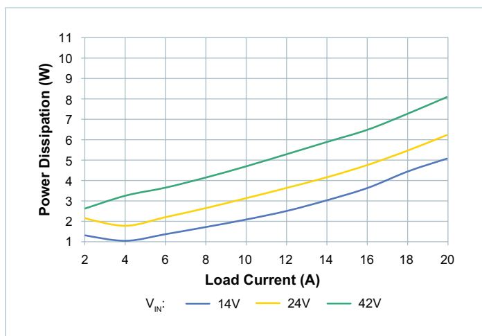
Figure 46 — System power dissipation, high trim, board temperature = -40°C
