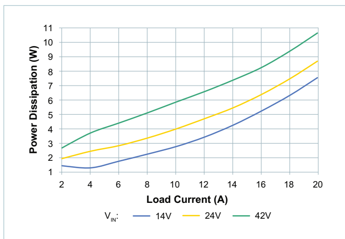
Figure 40 — System power dissipation, high trim, board temperature = 90°C
