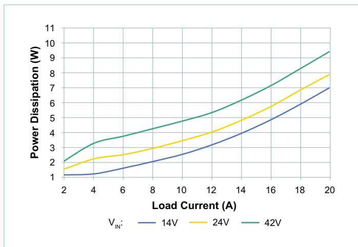
Figure 38 — System power dissipation, nominal trim, board temperature = 90°C
