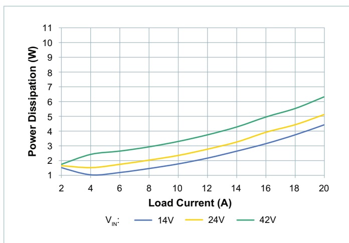
Figure 45 — System power dissipation, low trim, board temperature = -40°C
