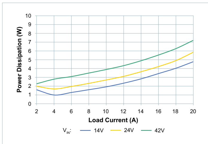
Figure 44 — System power dissipation, nominal trim, board temperature = -40°C
