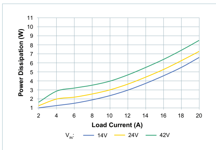
Figure 39 — System power dissipation, low trim, board temperature = 90°C
