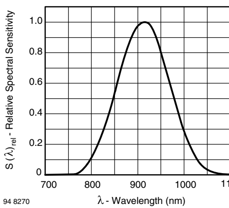
94 8270 Fig. 7 - Relative Spectral Sensitivity vs. Wavelength
