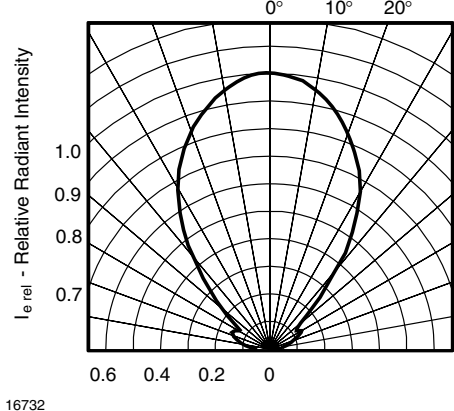
16732 Fig. 8 - Relative Radiant Intensity vs. Angular Displacement
