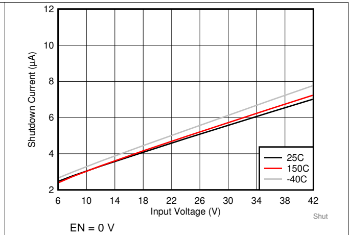
Figure 3. Shutdown Supply Current
