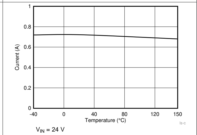
Figure 5. Low Side Current Limit
