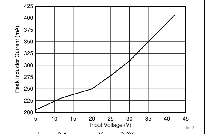
Figure 5. Low Side Current Limit
