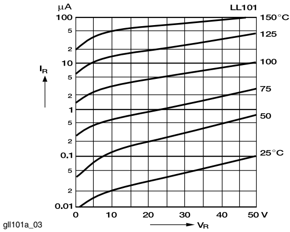
Fig. 3 - Typical Variation of Reverse Current at Various Temperatures
